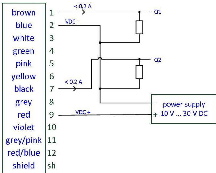
Figure 5: Wiring of Q1, Q2
