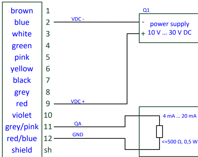
Figure 6: Wiring of QA
